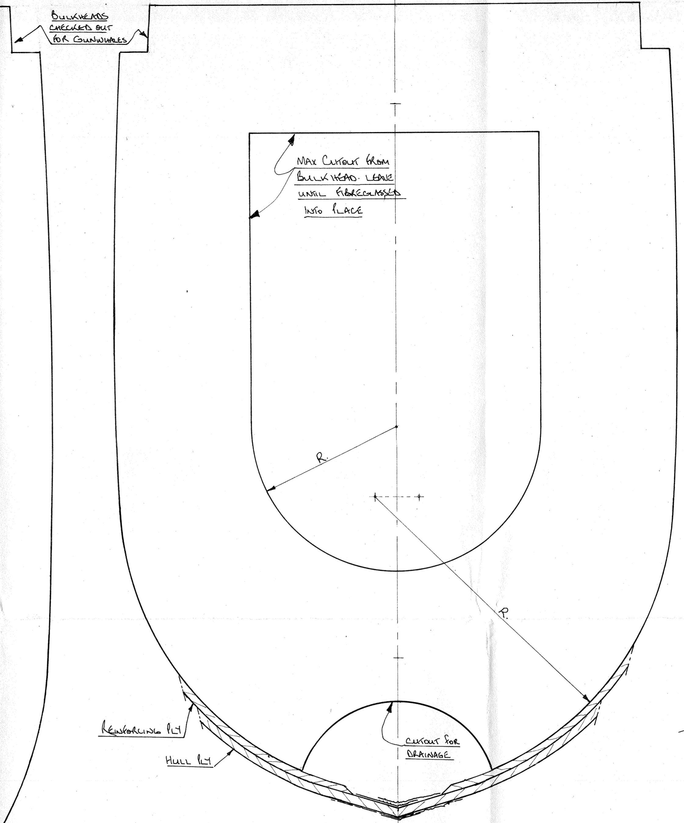
BULKHEAD AT REAR BEAM
